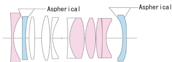
Abnormal partial dispersion lens
